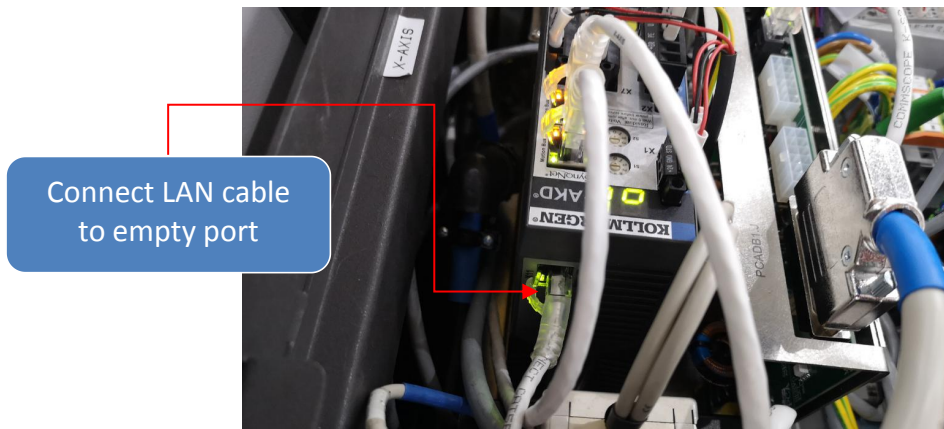
Figure 4 Connect LAN Cable to X-Axis AKD Kollmorgen Drive
