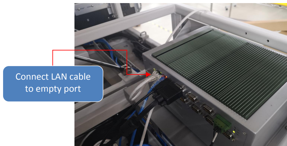
Figure 3 Connect LAN Cable to Atom PC on board LAN port
