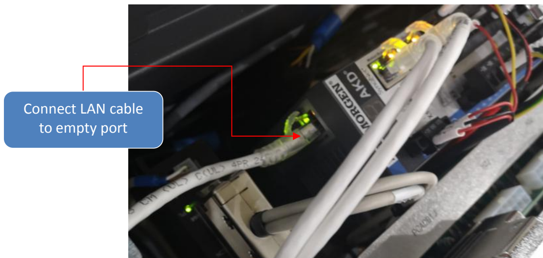
Figure 17: Connect LAN Cable to Y-Axis AKD Kollmorgen Drive
